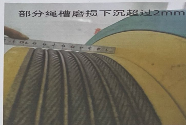
曳引轮
